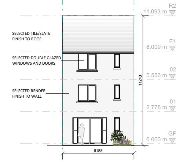
⑦ H08 Rear Elevation (MT) 1 : 200
