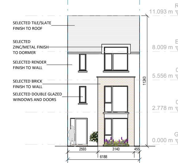
⑥ H08 Render Front Elevation (MT) 1 : 200
