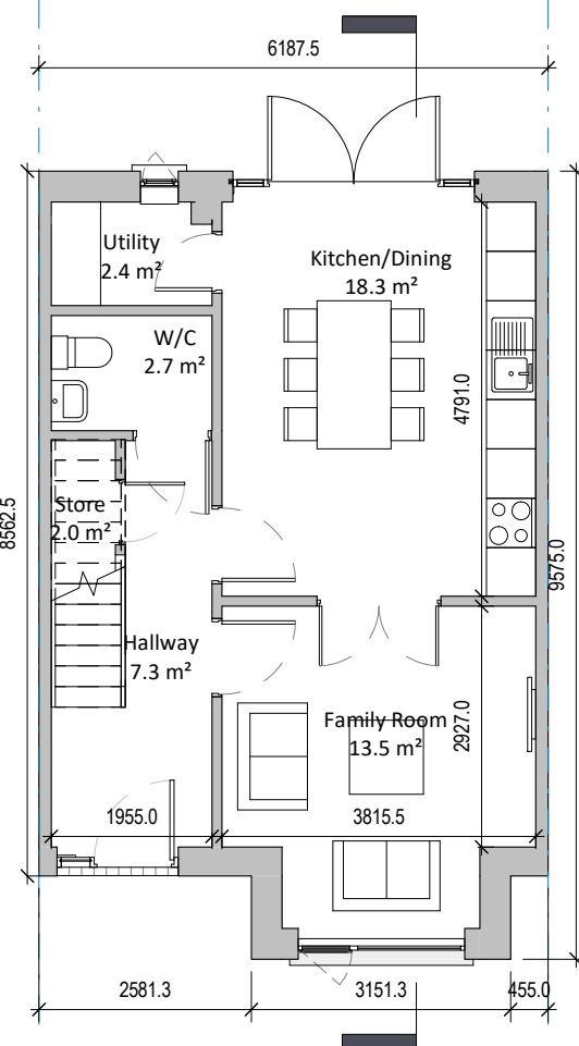
② H08 Level 00 (MT) 1 : 100
